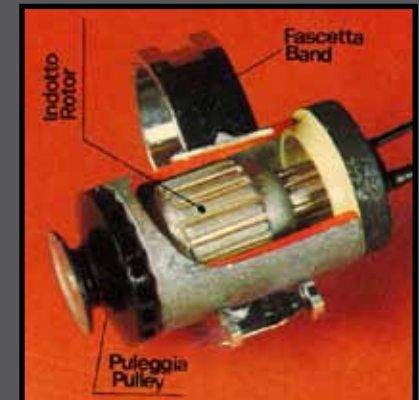
Dynamo
