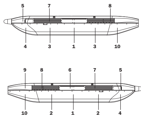
DECALS AN/ALQ99D
