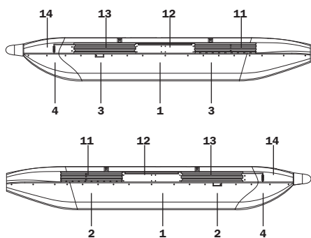
DECALS AN/ALQ99F
