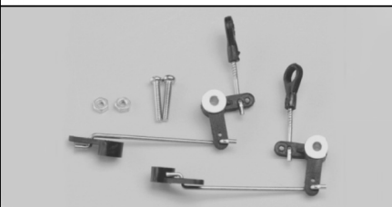
508129 Servo arm set Anlenkungs-Set BIG EC-135
