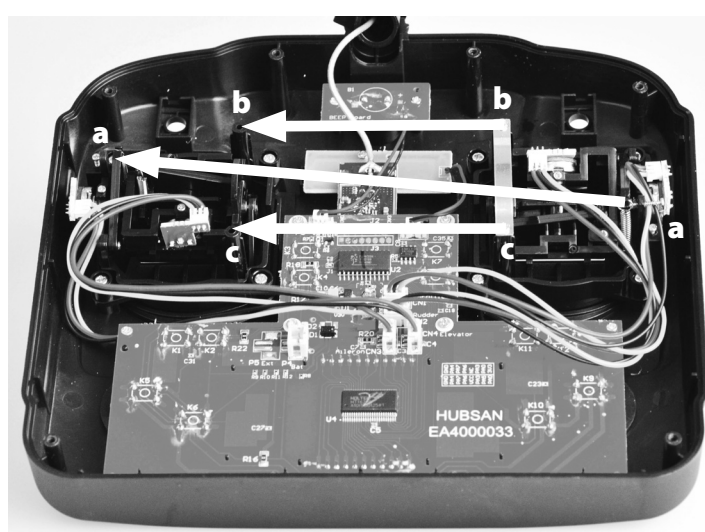
Unscrew screws a, b, c and move screw b, c and the spring to the other side. Fix it with the screws, and test if the stick moves smooth.
