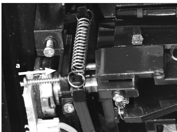
Important: Lift the arm and insert screw a from the left side.
