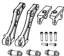
500405904 Spoilerhalter-Set Wing mount posts kit
