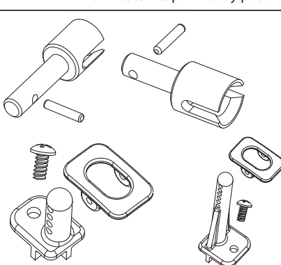
50 040 5339 Diff-Mitnehmer + Karosseriepin Diff outdrive pin + body post
