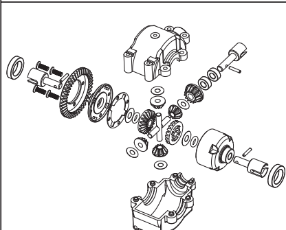
50 040 5326 Differenzial v/h komplett Diff gear box unit f/r complete
