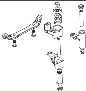
50 040 5332 Servosaver Set Servo saver unit
