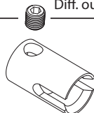
50 040 5279 Differenzialzapfen Set Diff. outdrive set, M4 x 4 mm
