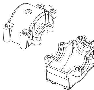
50 040 5284 Diffgehäuse Diff gear upper/lower
