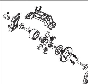
50 040 5319 Zentraldifferenzial komplett Centre differential unit complete
