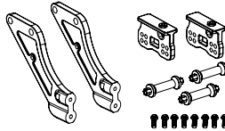
500205943 Servosaver-Unit Servosaver-Einheit
