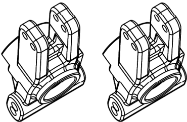
500405341 Rear hub carrier left/right (2) Achsschenkel hinten l/r (2)
