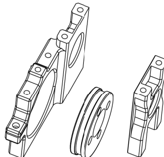
500405230 Diff mount set Diff-/Motorhalteset
