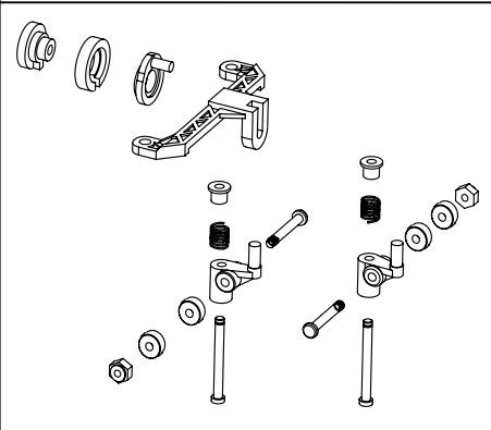
50 040 8063 Vorderachse X-24 Front axle X-24
