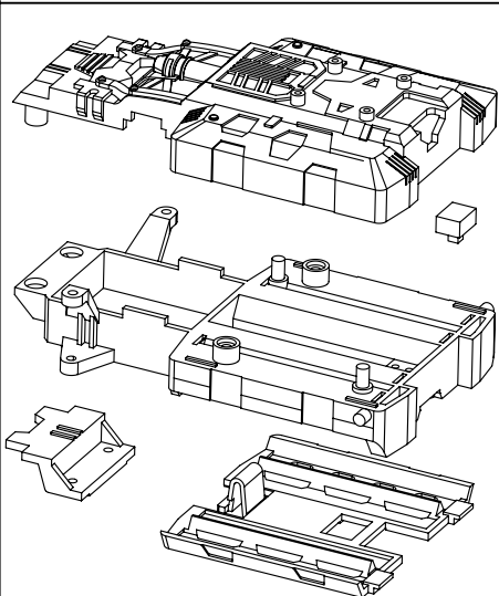
50 040 8062 Chassis-Set X-24 Chassis kit X-24
