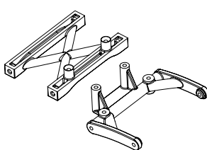
500405794 Chassis Verbinder A hinten (1) / Chassis holder A
