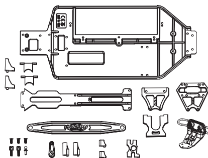
500405422 Chassis/Anbauteile-Set Chassis plates replacement set
