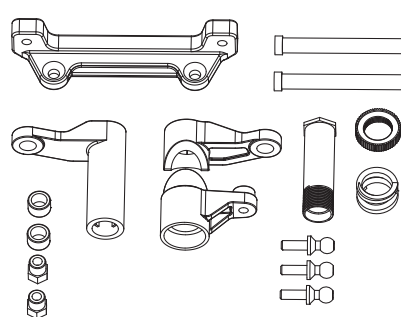
50 040 5360 Servosaver/Lenkeinheit Servosaver/steering set
