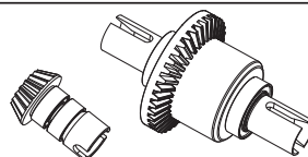
50 040 5363 Differenzial hinten komplett Diff complete rear
