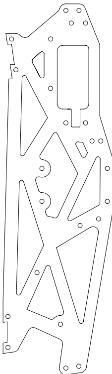
205120 Aluminium Chassis / Chassisplatten
