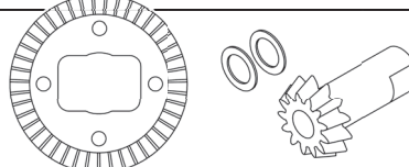
205355 Pinion gear 13 T steel + 43 T Kegelritzel 13 Z Stahl + Kegelrad 43 Z
