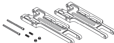
205325 Lower rear suspension alu blue Querlenker unten hinten Alu blau
