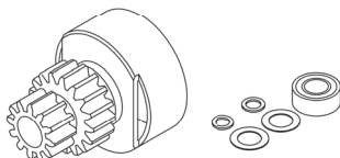
205284 2 Speed pinion gear 2-Gangritzel 12 Z + 17 Z
