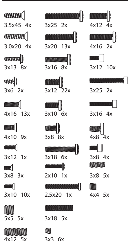
500205807 Screw set 1 Schraubenset 1
