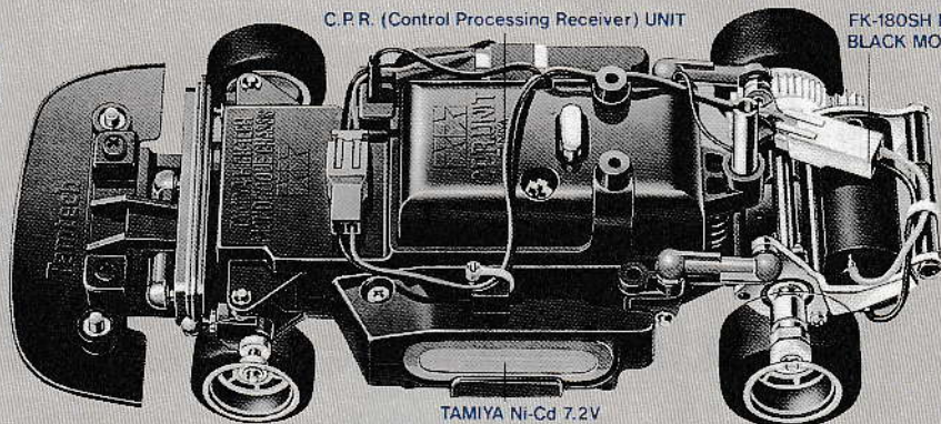
TAMIYA Ni-Cd 7.2V TAMPACK BATTERY
